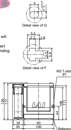
Cable track for user wiring Dimensions of section (type M)
