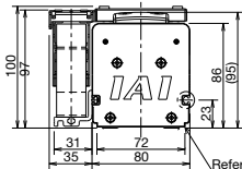
Cable track for user wiring Dimensions of section (type M)
