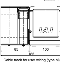
Cable track for user wiring (type M)
