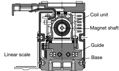
■ Section View of Shaft Type
