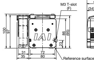
Reference surface
