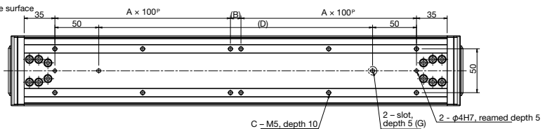
Cable track for user wiring (type M)
