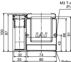
Cable track for user wiring (type M)
