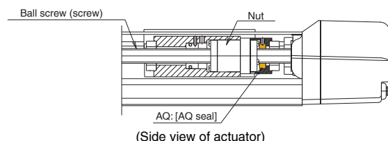
(Side view of actuator)
